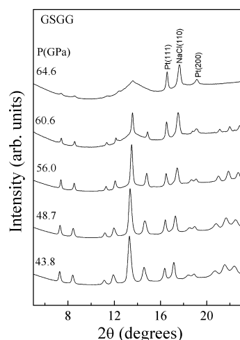
Figure 2. Representative angle-dispersive X-ray diffraction patterns (wavelength \lambda = 0.6199 \text{\AA} ) of GSGG during compression at room temperature. NaCl was used as the pressure-transmitting medium.
