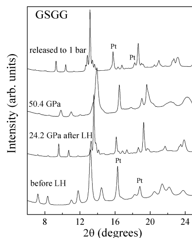
Figure 3. Representative angle-dispersive X-ray diffraction patterns (wavelength \lambda = 0.6199 \text{\AA} ) of GSGG after laser heating. The diffraction patterns before laser heating are given for comparison.
