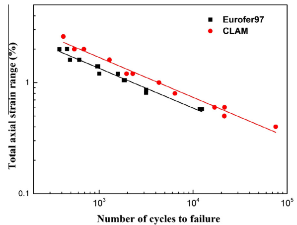
Fig. 3. S–N curves of CLAM and Eurofer97 specimens at RT.
