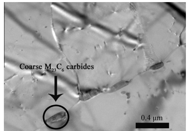
Fig. 7. Coarse M_{23}C_6 carbides on subgrain boundaries.
