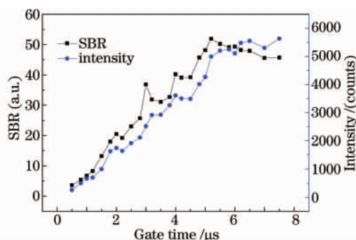
图 4 钾 769.90 nm 谱线的 SBR 和强度随门宽的变化 Fig. 4 SBR and intensity of K 769.90 nm spectral line versus gate time
