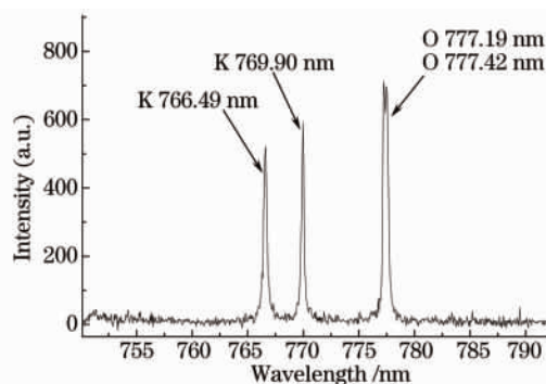
图 2 钾在 755~790 nm 波长范围内的等离子体发射光谱 Fig. 2 Plasma emission spectrum of potassium within the range of 755~790 nm
