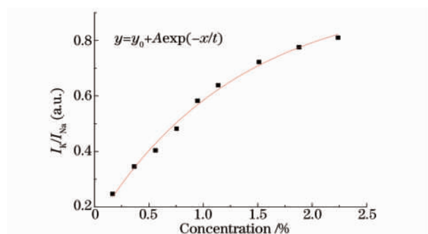
图 5 钾 LIBS 谱线强度随其浓度变化的关系 Fig. 5 Relationship between LIBS intensity of potassium and concentration
