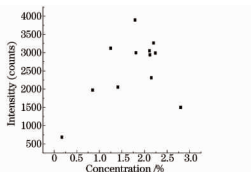
图 7 不同土样钾元素质量分数与其对应的光谱强度 Fig. 7 Spectral intensity of potassium corresponding to its mass fraction in different types of soil
