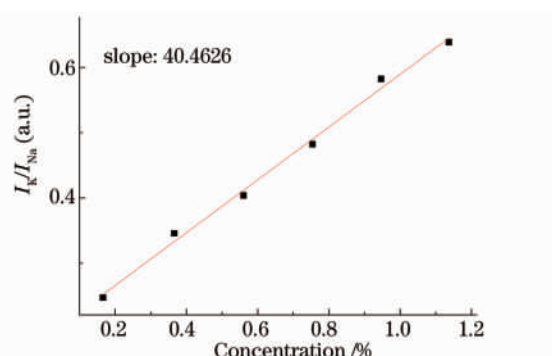
图 6 钾元素浓度较低时其谱线强度随浓度变化关系 Fig. 6 Relationship between LIBS intensity of potassium and concentration when concentration is low
