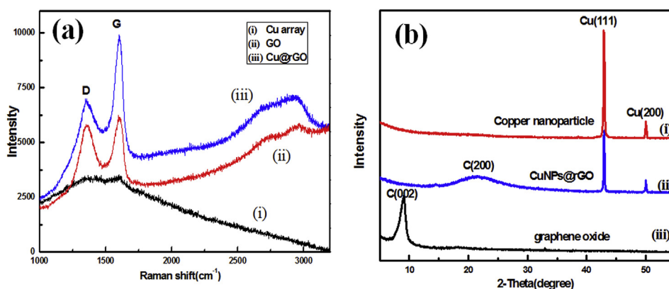
Fig. 5. (a) The three curves of Raman spectra from down to up correspond to samples of Cu NPs (i), GO (ii) and Cu@rGO (iii) respectively. (b) XRD diffractograms of the synthesized copper nanoparticles (i), the Cu@rGO (ii) and graphene oxide (iii).
