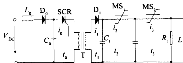
Fig. 1 A new type charge and discharge circuit schematic diagram of Ti:sapphire laser power supply
