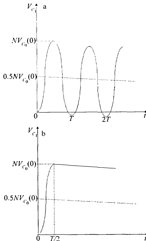
Fig. 3 Charge waveform of resonant pulsed transformer a—the resonant charge waveform of capacitor C_1 without diode D_1 b—the voltage waveform of capacitor C_1
