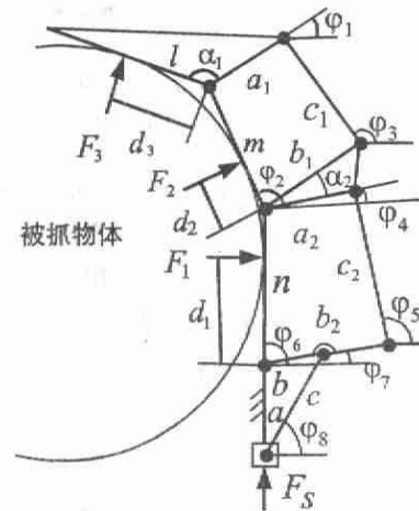
图 2 形状自适应欠驱动手指机构 Fig. 2 The shape self-adapting underactuated finger
