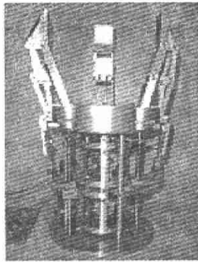
图 1 基于锥齿轮差动机构的欠驱动手爪 Fig. 1 Underactuated robot hand based on cone gear differential mechanism
