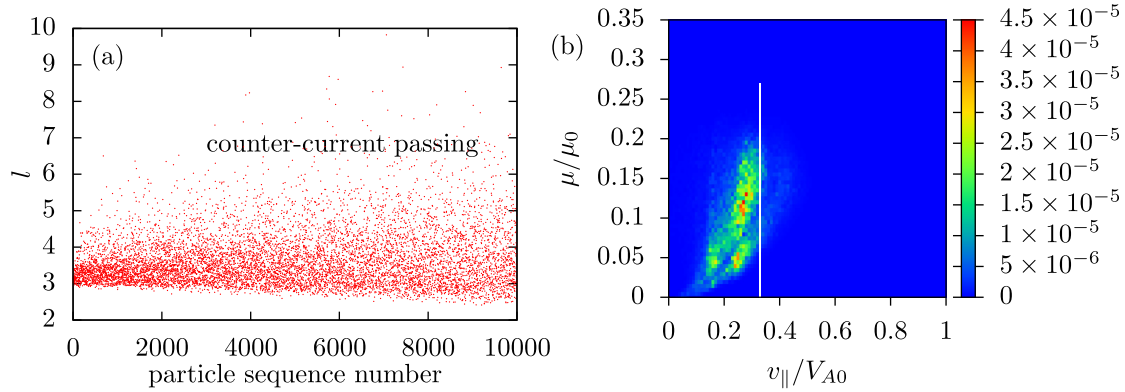
FIG. 10. (a) The values of the resonance number l of the top 10000 markers with a large value of |\delta f| . (b) Contour of averaged |\delta f| on the (v_{\parallel}, \mu) plane in the linear stage of the mode evolution, where the white line indicates the location v_{\parallel} = V_{A0}/3 .
