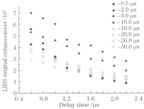
图 5 在不同两脉冲间隔下,信号强度随采集延时的变化 Fig. 5 Signal intensity versus the gate delay time at different delays between the two pulses
