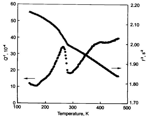
Fig.3 A typical example of internal friction and shear modulus induced by the presence of oil film containing 0.7% S deposited on a steel substrate, the peak at around 270 K and the corresponding variation of the shear modulus to be caused by the glass transition of the oil and the high temperature peak to be the SK peak caused by the substrate
