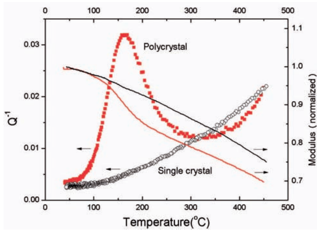
Fig. 1. Internal friction and normalized modulus of the Mg polycrystal and single crystal measured at 1.0 Hz
